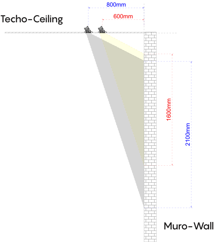
Vista lateral-Side view
